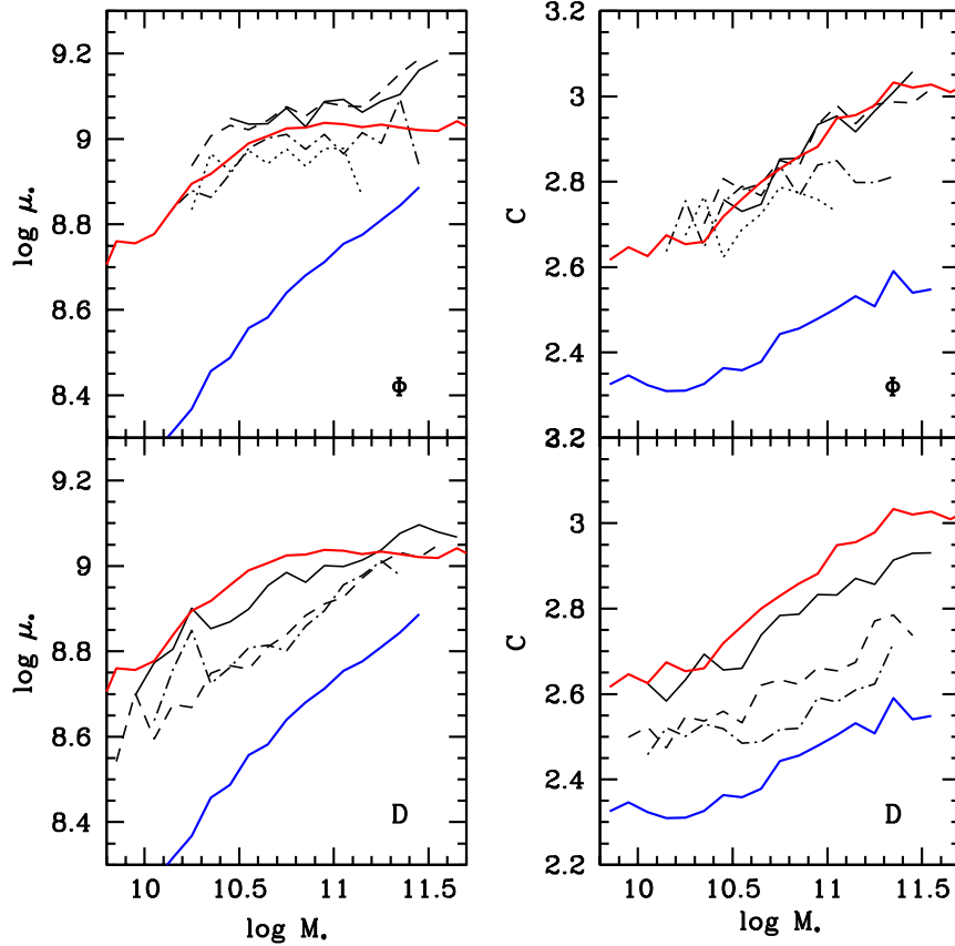
Figure 11: Trends in the \mu_* - M_* and C - M_* relations for AGN hosts as a function of angle parameter \Phi and distance D from the locus of star-forming galaxies. Blue and red lines show the median relations for ordinary late- and early-type galaxies. The black line types are solid, dashed, dashed-dotted and dotted in order of decreasing \Phi (top) and decreasing D (bottom).
